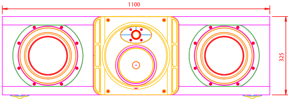
2-FRONT
